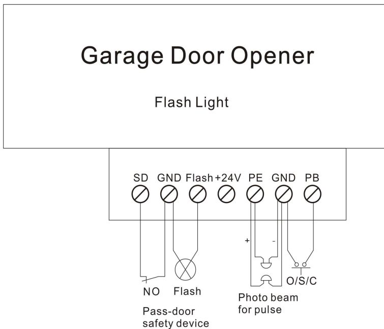
ASS. Terminal connection
